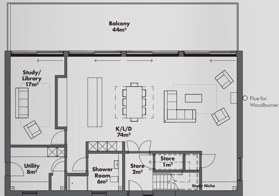
GROUND FLOOR
